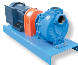
BU1533 Electric Motor Model (Long Coupled Version Shown)
