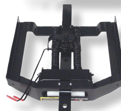
Cush'n Combo Hitch Frame (Flat Bar)
