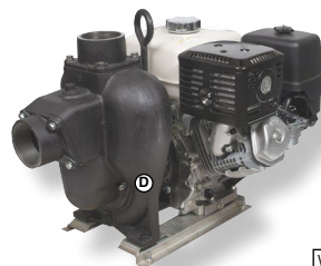
Gas Engine No. 1542P-65SPM with Roll Cage
